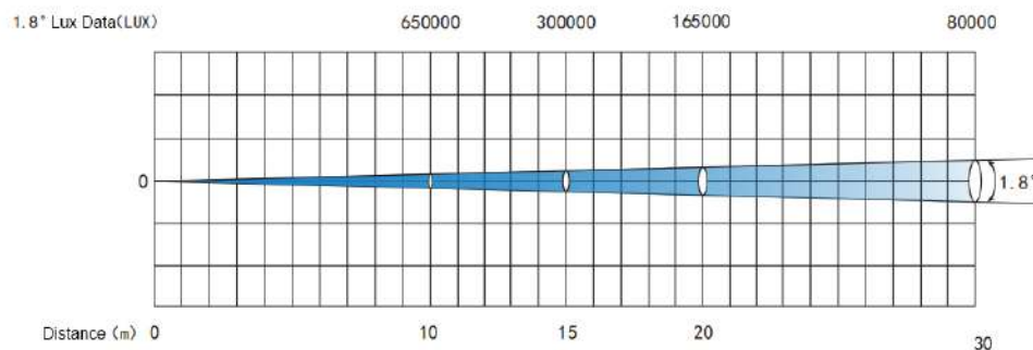
420W Beam Moving Head
